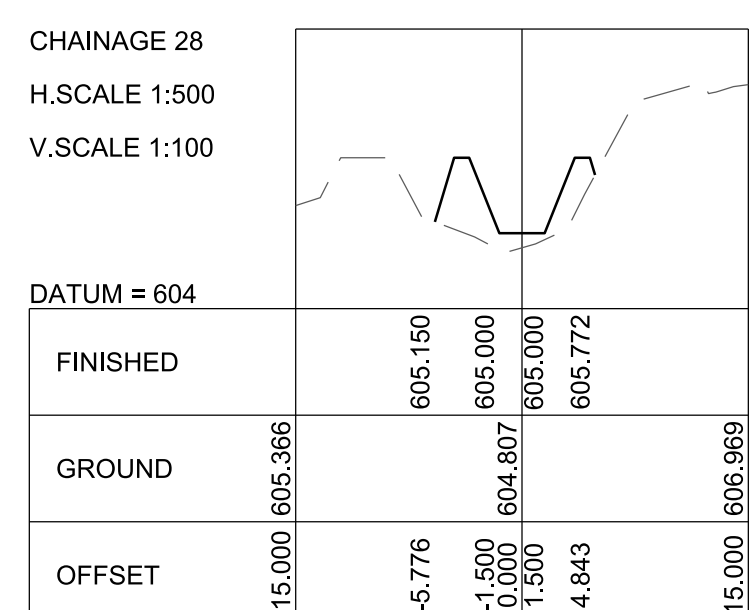
CROSS SECTION : OFFTAKE CANAL C1 SCALE : AS SHOWN
