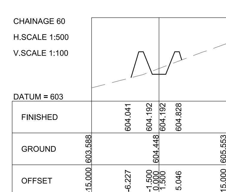
CROSS SECTION : OFFTAKE CANAL C3 SCALE : AS SHOWN
