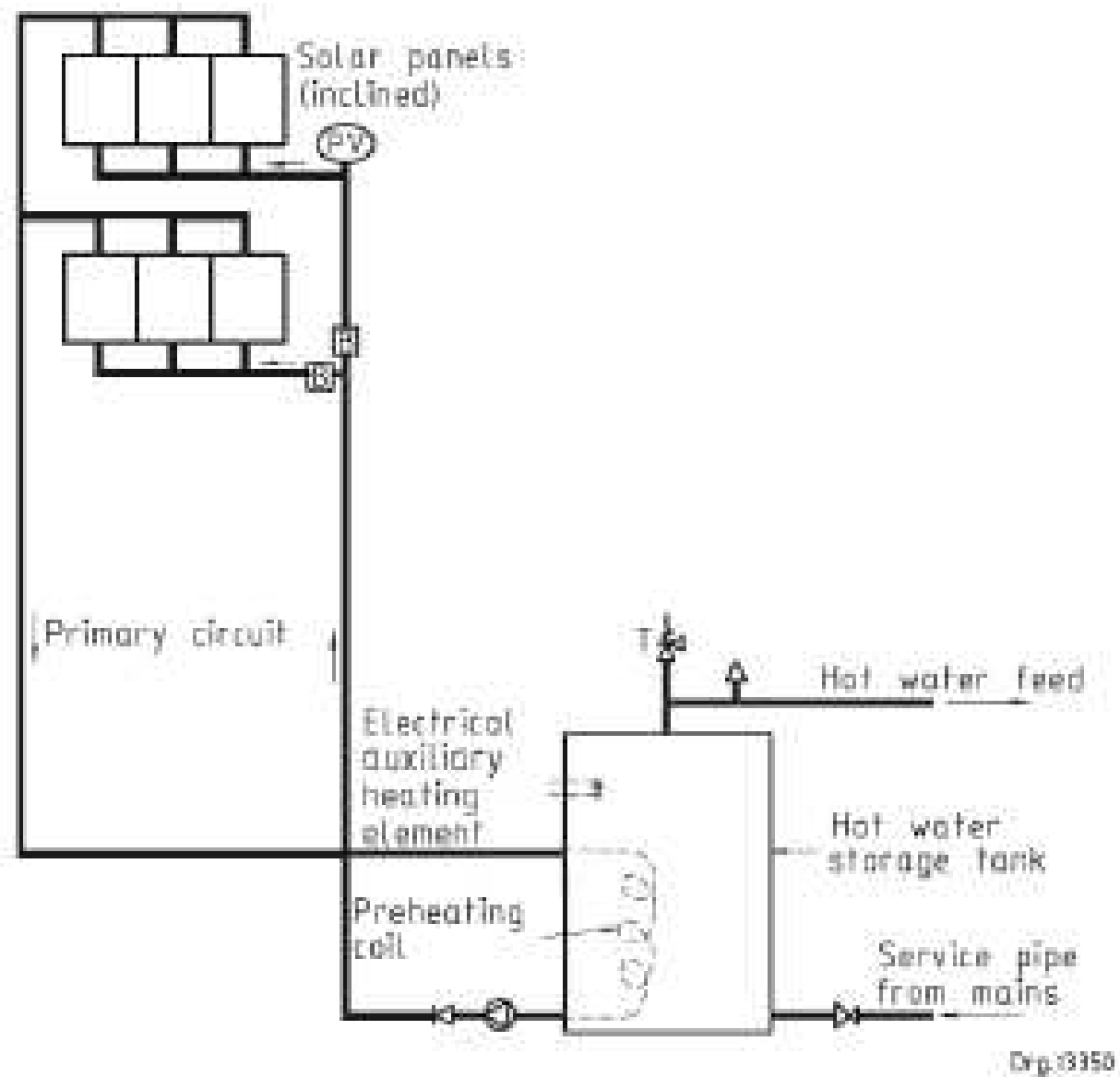
Figure 4 — Pumped indirect solar water system
