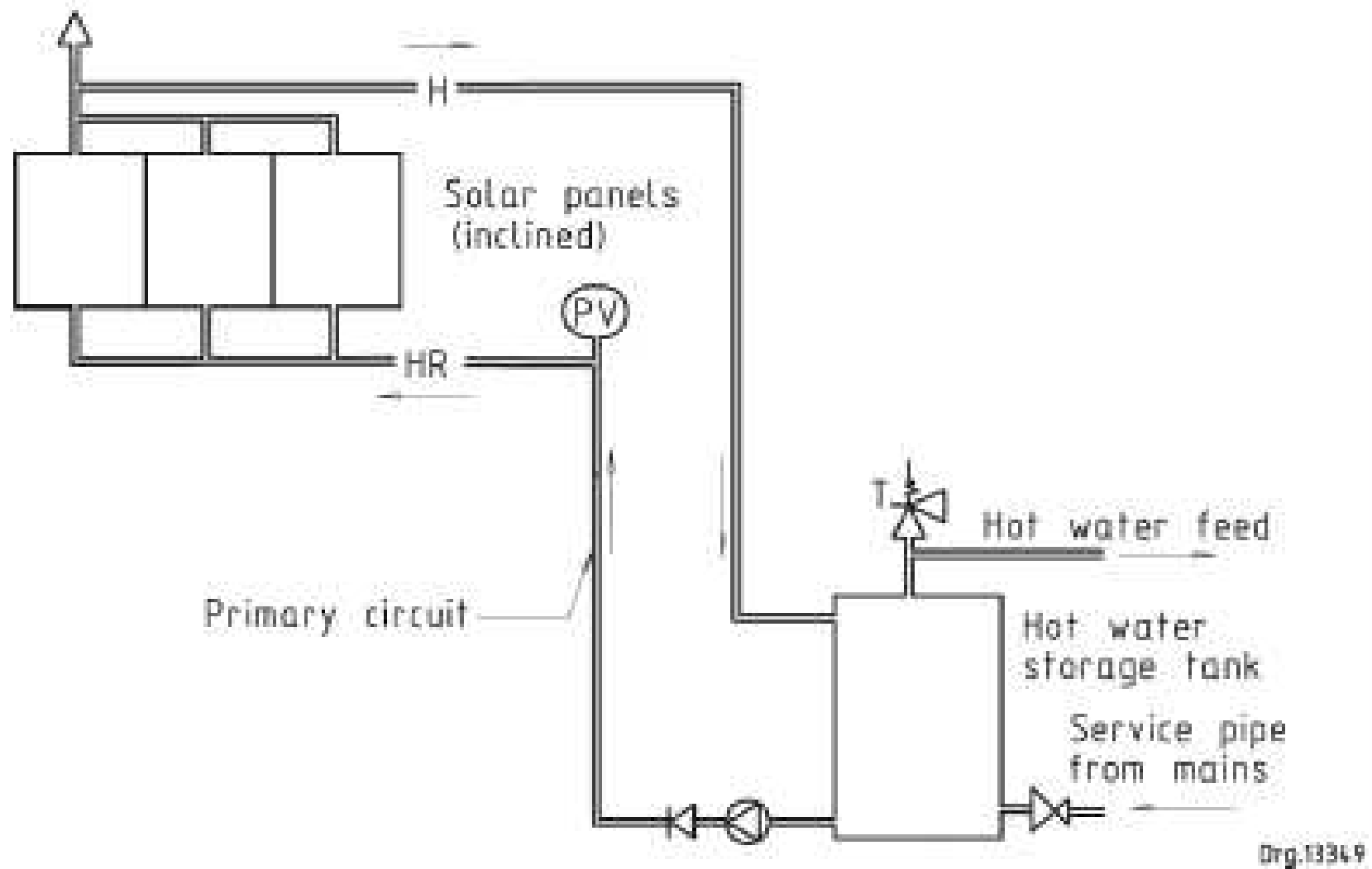
Figure 3 — Pumped direct solar hot water system
