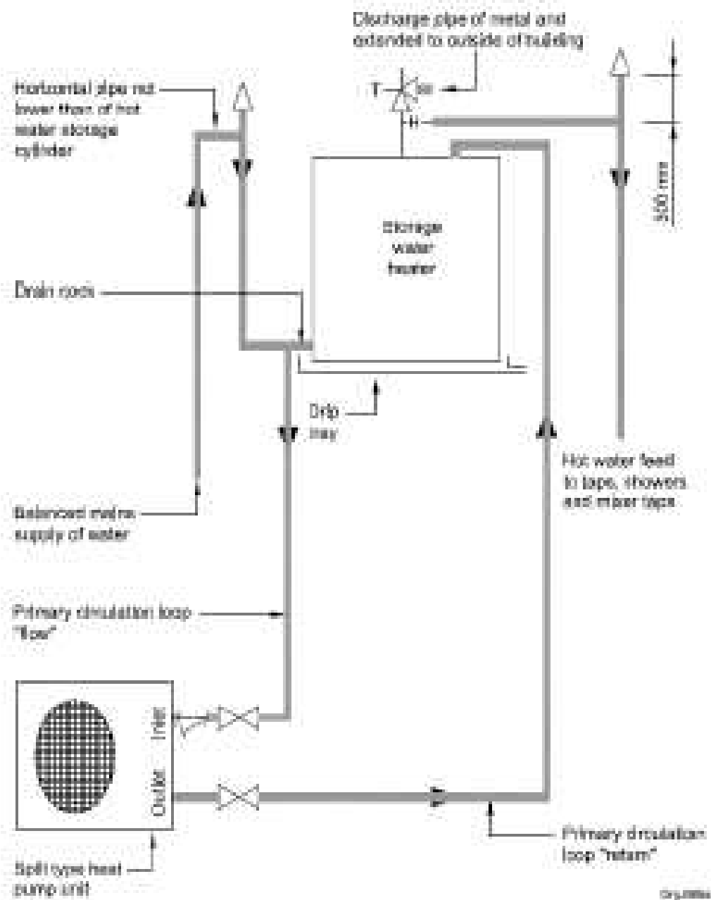
Figure 2 — Split type heat pump unit with an integrated pressure and temperature safety valve and hot water outlet
