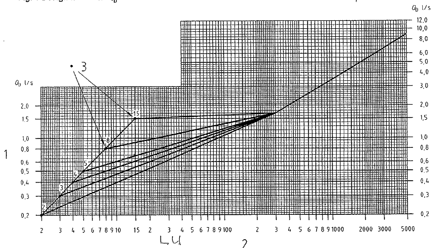
Fig. 1 Design flow rate Q_D in l/s for standard installations in relation to total flow rate Q_T in LU
