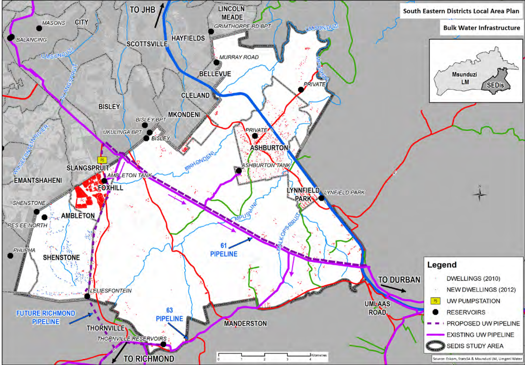
Figure 1: Bulk Water Infrastructure
