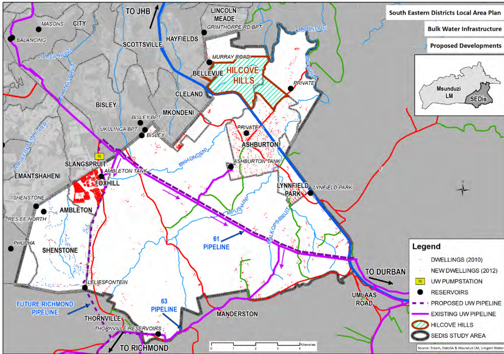
Figure 2: Bulk Water Infrastructure and Proposed Developments
