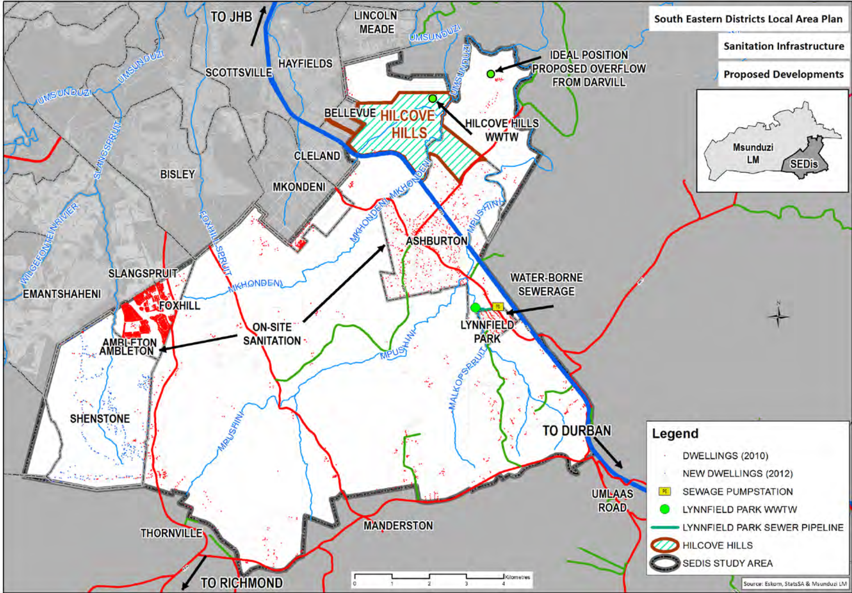
Figure 4: Bulk Sanitation Infrastructure and Proposed Developments
