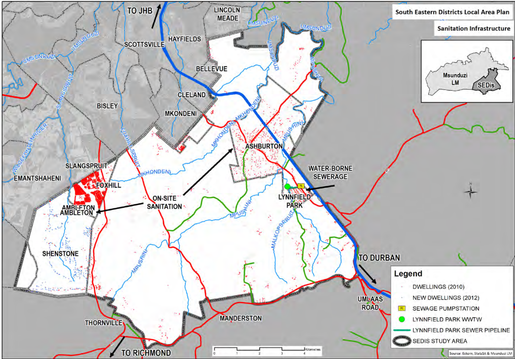
Figure 3: Bulk Sanitation Infrastructure
