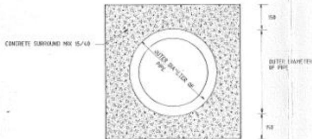
DETAIL OF CONCRETE ENCASED PIPE
