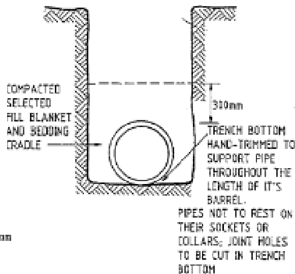
d. RIGID PIPE ON CLASS D BED
