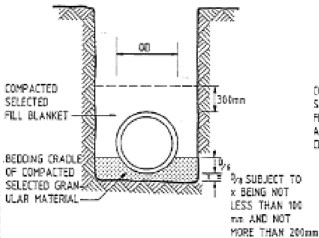
c. RIGID PIPE ON CLASS C BED
