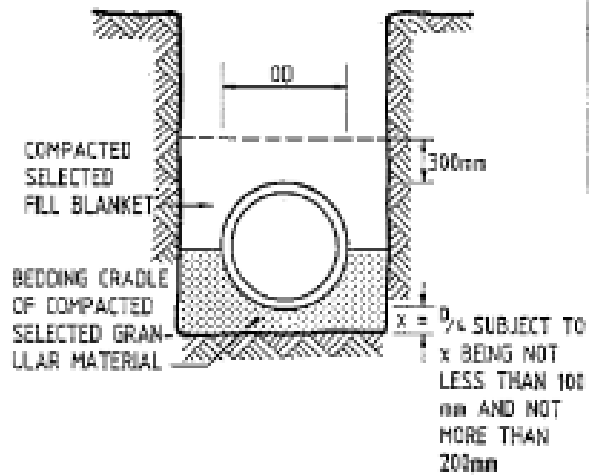
b. RIGID PIPE ON CLASS B BED
