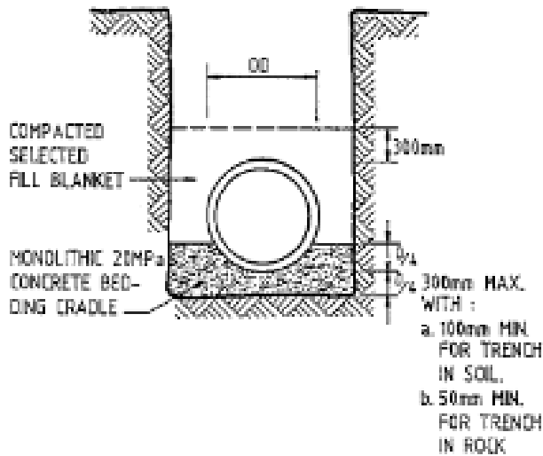
c. RIGID PIPE ON CLASS C BED
